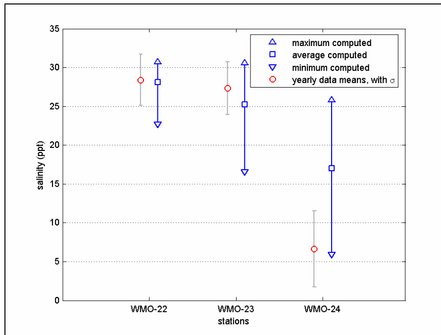
Figure VI-5. Comparison of measured and calibrated model output at stations in Namskaket Creek. Stations labels correspond with those provided in Table VI-1. Model output is presented as a range of values from minimum to maximum values computed during the simulation period (triangle markers), along with the average computed salinity for the same period (square markers). Measured data are presented as the total yearly mean at each station (circle markers), together with ranges that indicate \pm one standard deviation of the entire dataset.
