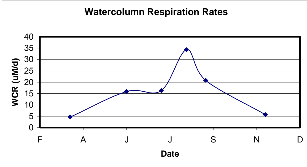
Figure VII-1. By example, average water column respiration rates (micro-Molar/day) from water collected throughout the Popponeset Bay System (Schlezinger and Howes, unpublished data). Rates vary ~7 fold from winter to summer as a result of variations in temperature and organic matter availability.
