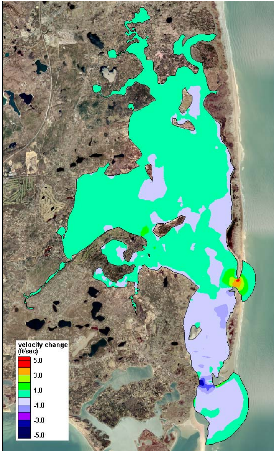
Figure 17. Contour plot showing computed maximum flood velocity change (post minus pre) between model runs of 2004 and 2007 inlet configurations, both using the November 2007 offshore boundary condition.
