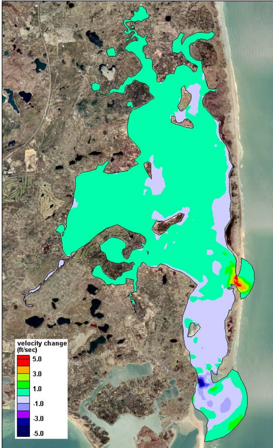
Figure 16. Contour plot showing computed maximum ebb velocity change (post minus pre) between model runs of 2004 and 2007 inlet configurations, both using the November 2007 offshore boundary condition.
