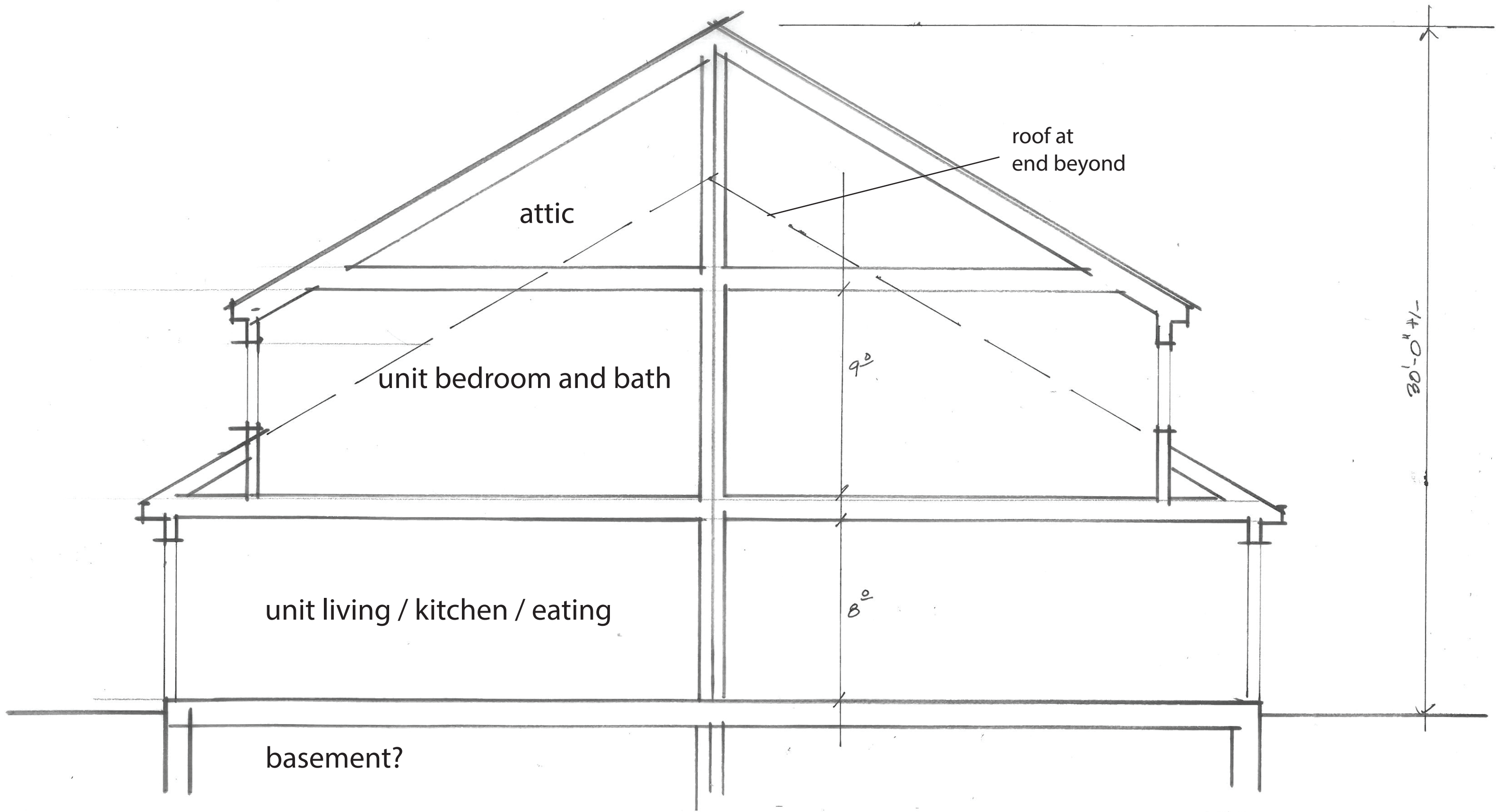
'Barn' - Schematic Cross-Section
